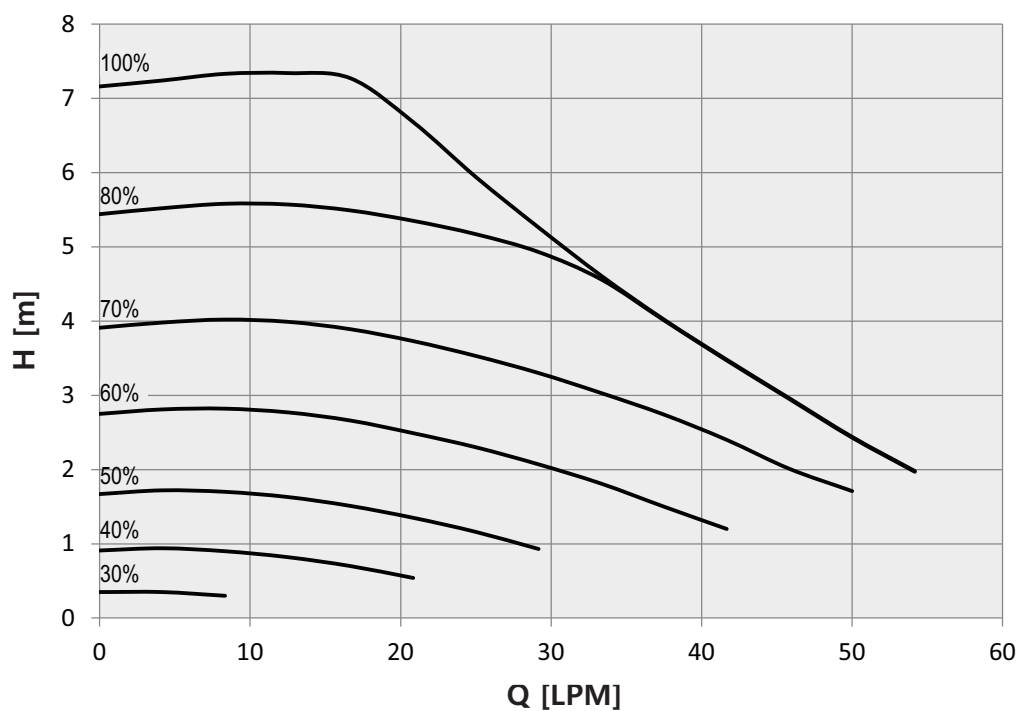
Q-H Chart
