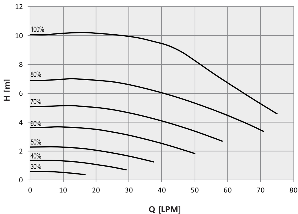
Q-H Chart
