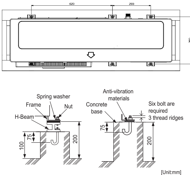
Foundation bolt executing method
