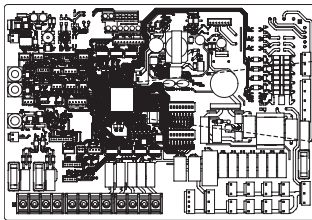
Innen-PCB
