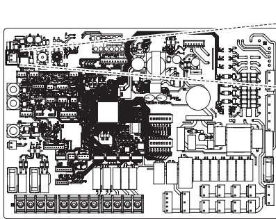
Innen-PCB
