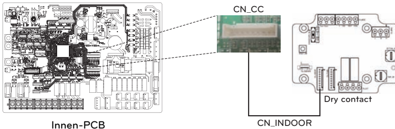
Innen-PCB
