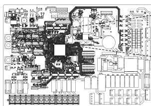
Innen-PCB
