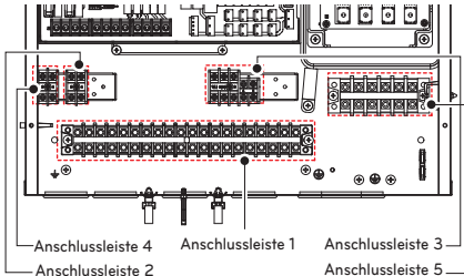
Phase 1(Ø)
