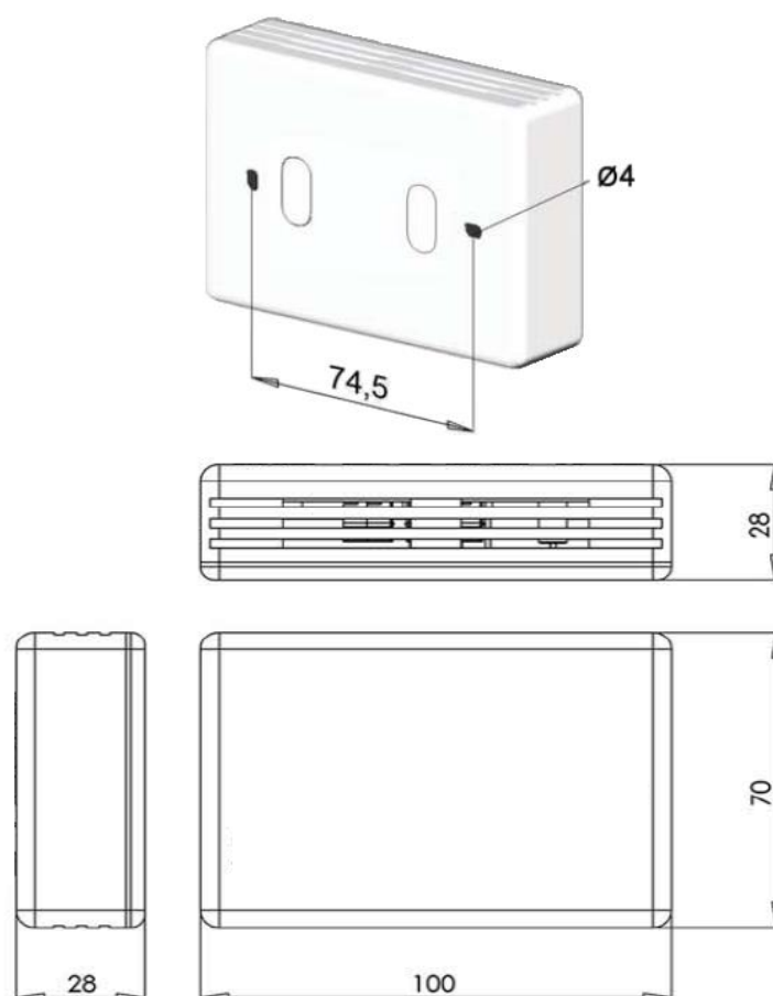
Figure 5.1 PA-AW-KNX-1 dimensions (mm)
